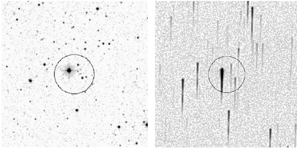
Fig. 3. A comparison of the same field from the Digitized Sky Survey (DSS; direct images) and DFBS (spectral images). 2D spectra significantly facilitate the search and identification of objects.
